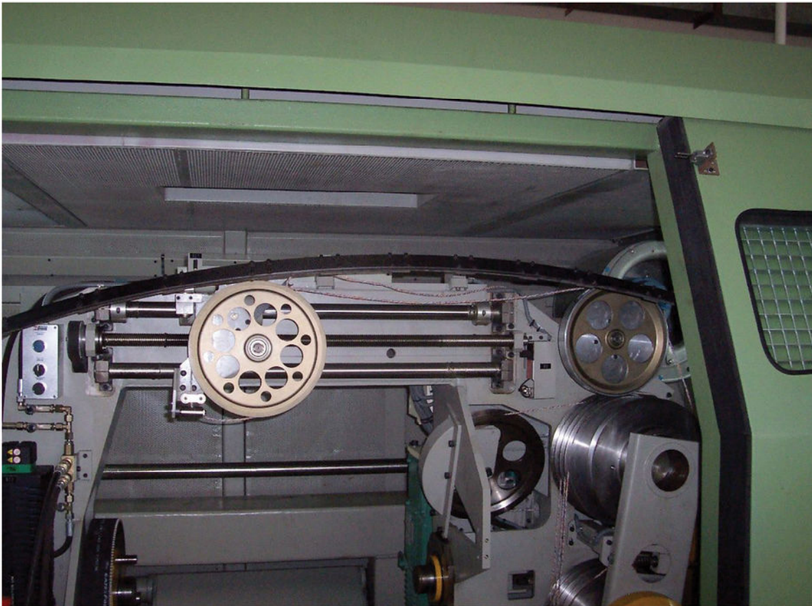
Fig.15 The $800,000 precision twisted-pair machine
