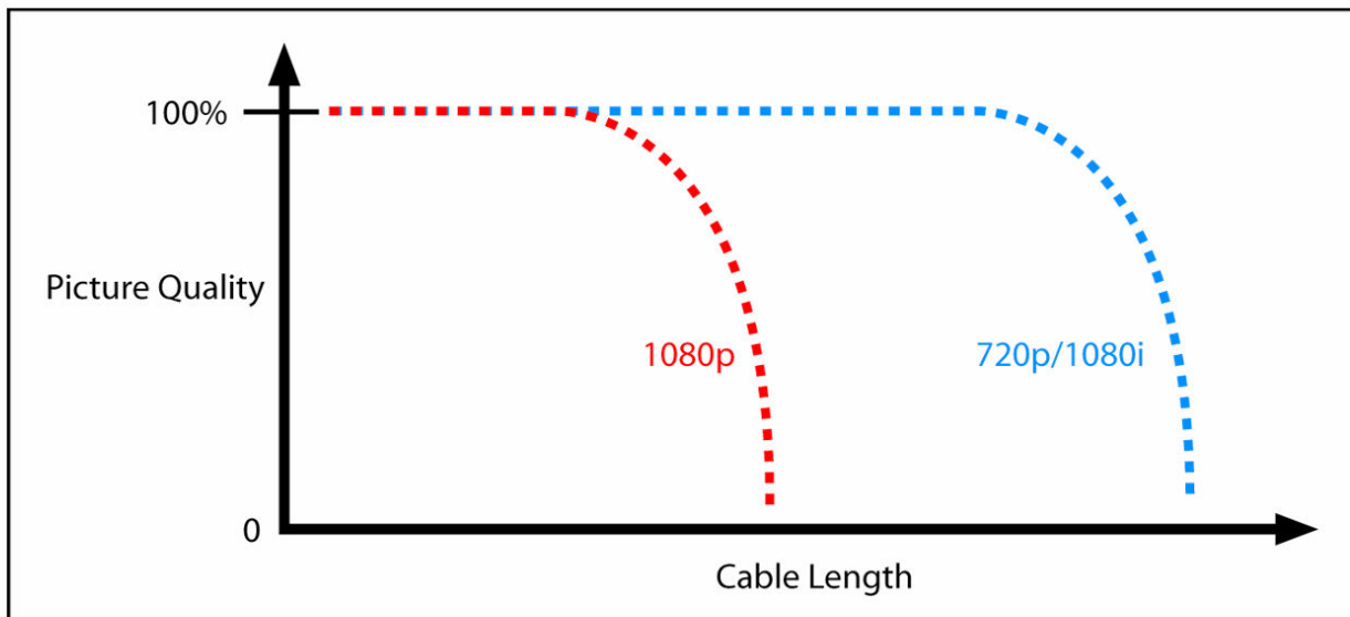
Fig.13 The edge of the “cliff” of a given cable varies by signal rate. The max distance of 1080p is only 1/2 of 1080i.
