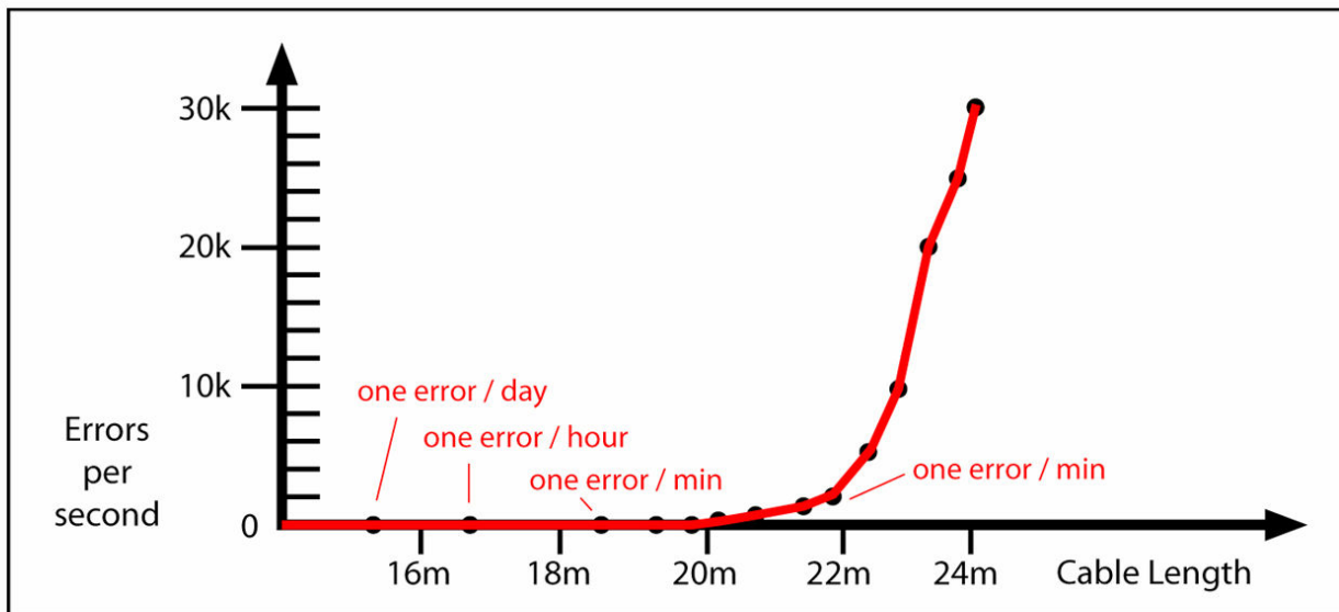
Fig.11 BER test also shows the “cliff” effects.
