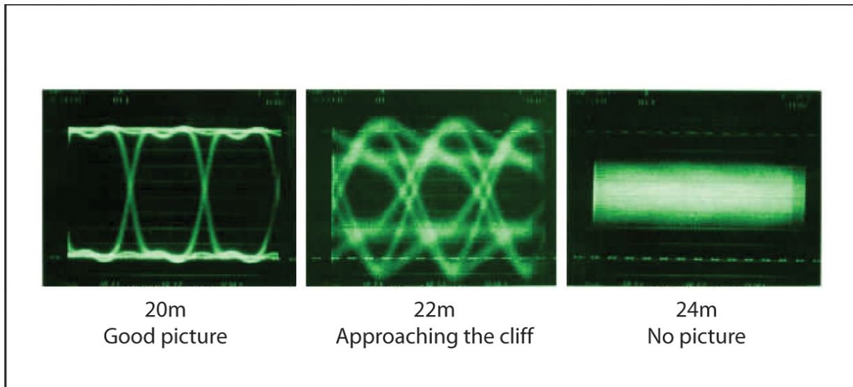
Fig.10 “Eye pattern” test shows the wave forms of the digital signal (bits) visually. It also shows the “cliff” effects.
