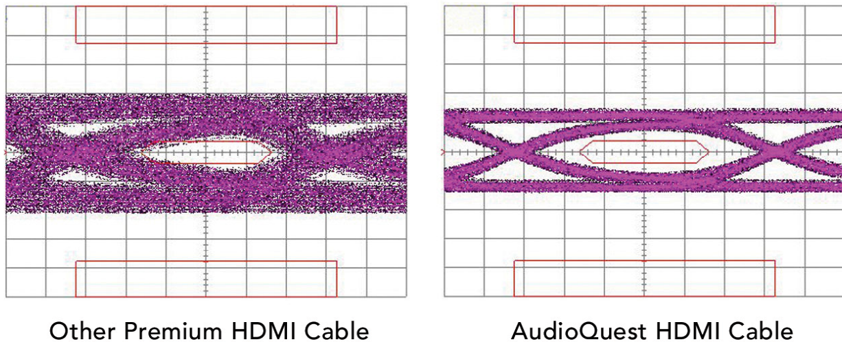
Fig.14 Eye pattern test results
