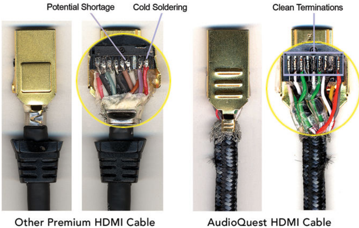
Fig.17 Soldered vs. crimped connection
