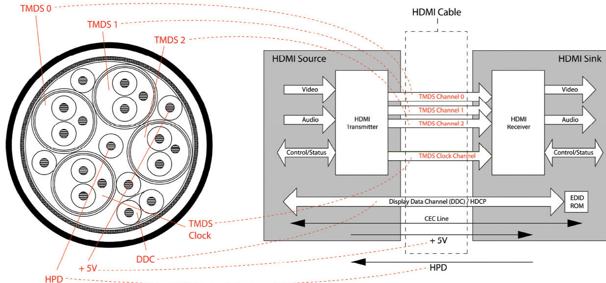
Fig.1 Components inside a HDMI Cable
