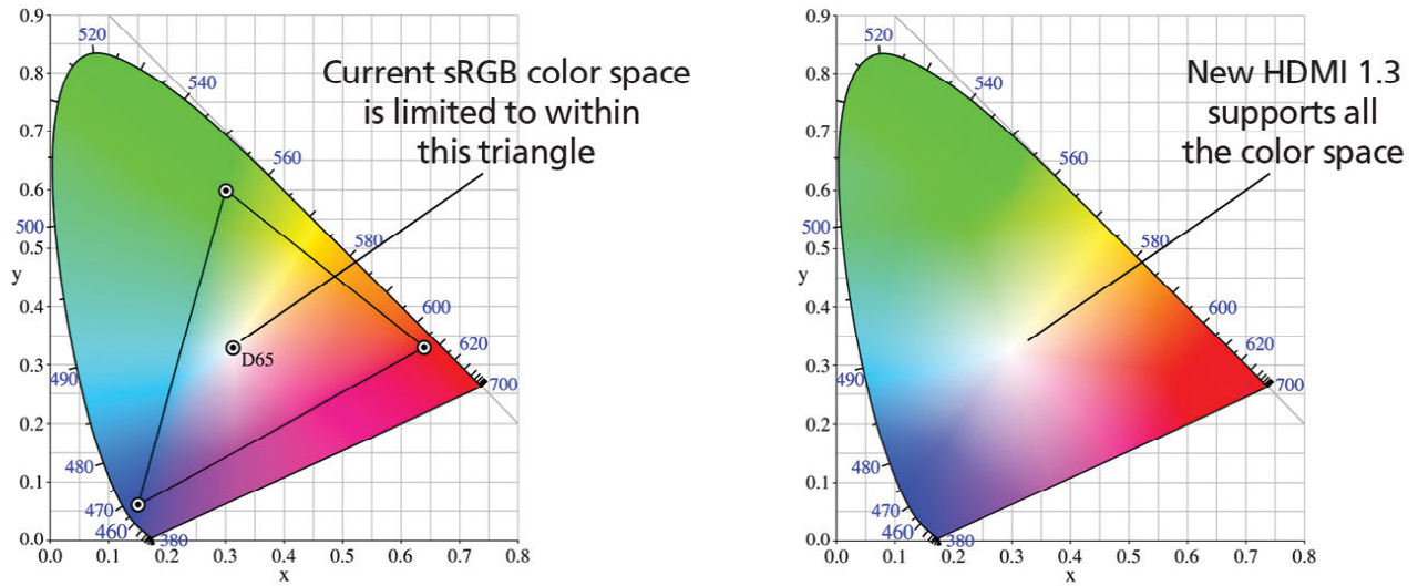
Fig.3 Wider Color Space
