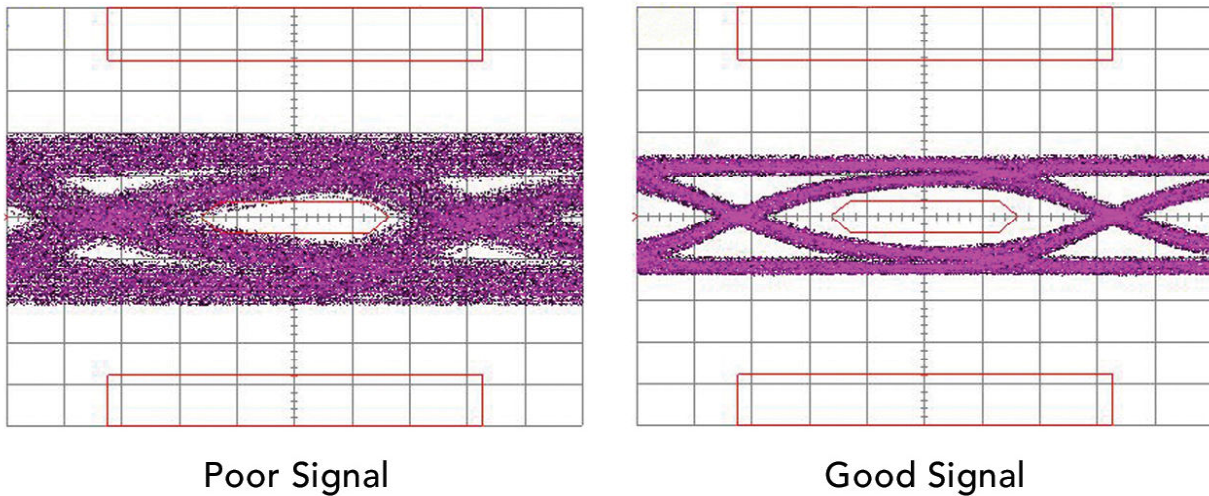
Fig.9 HDMI "Eye" patterns
